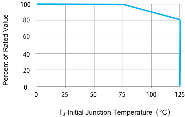
FIGURE 1 Peak Power Derating
